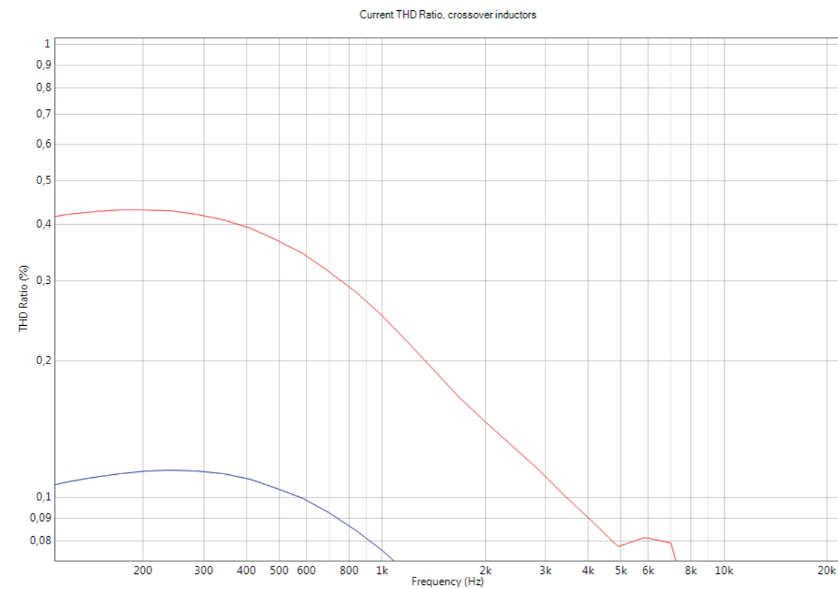
▲ The measurement illustrates a SMC-KORE inductor (— Blue) compared to an inductor with a conventional iron powder core (— Red). Both inductors are of 5.7 milli-Henry inductance, and in the measurement setup they are connected in series with a 4 Ohm resistor to create an appropriate load for the driving amplifier. The measurement shows that the SMC inductor reduces pass-band Total Harmonic Distortion (THD) by a factor of around 3.5 vs. a conventional iron powder core.
