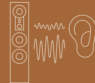
TIME COHERENCE
